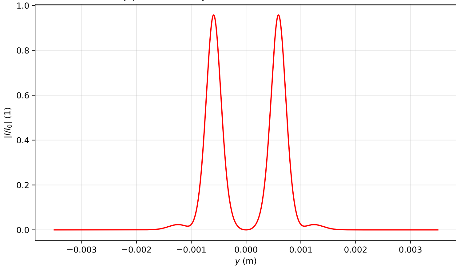
Intensity profile I(x=0, y, z=0.955)/I_0 , P_{in}=6.0P_{cr} , artificial time
